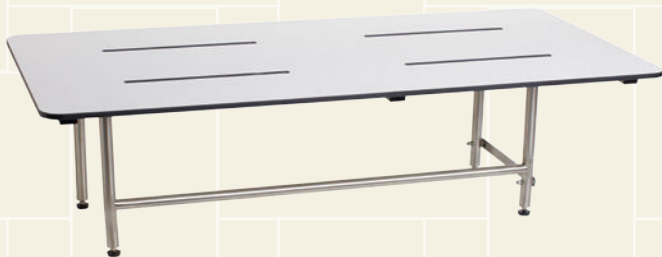
BENCH SEAT This bench shower seat with legs provides a phenolic top securely supported by a #304 stainless steel frame. Meets all federal specifications. LENGTH: 48" | DEPTH: 24"
